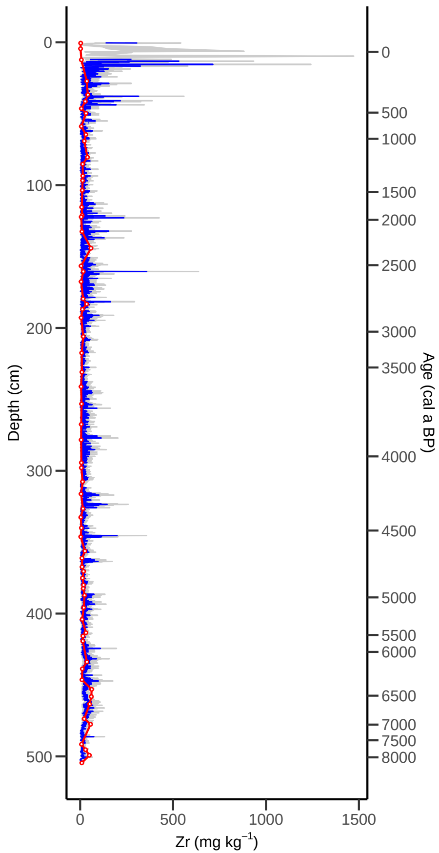
BI10: PLSR Zr Predictions with Confidence Interval
